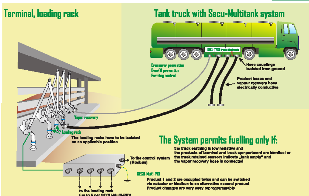
Simplified diagram Depot
