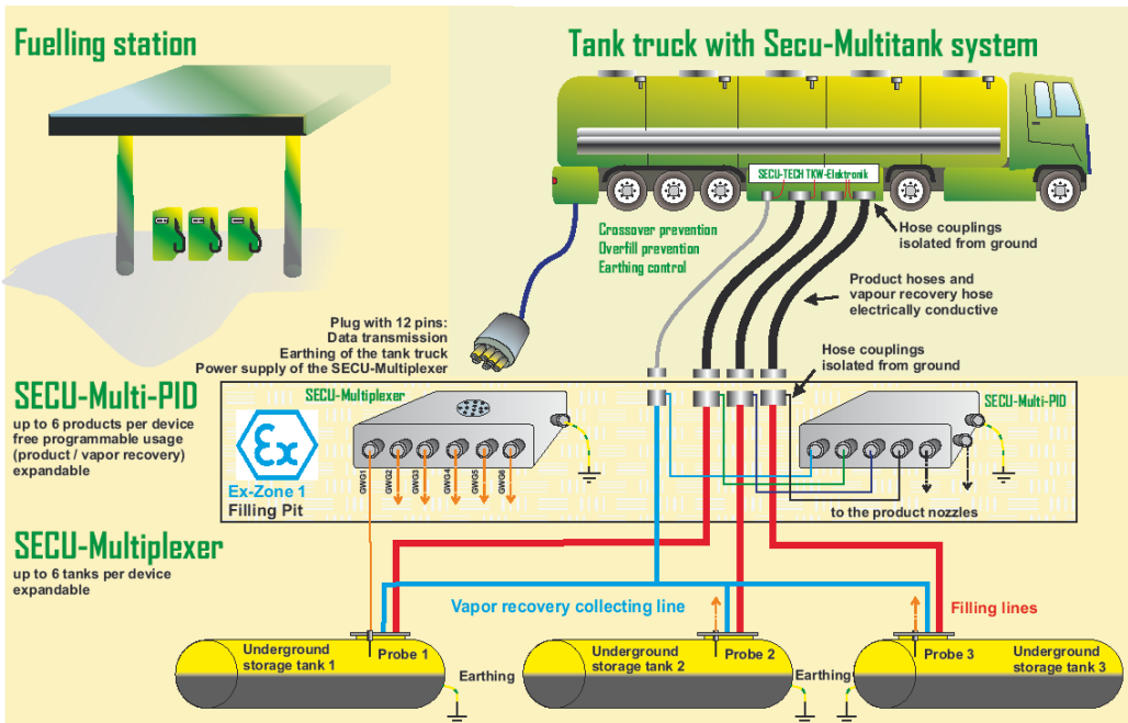
Simplified diagram Fuelling station
